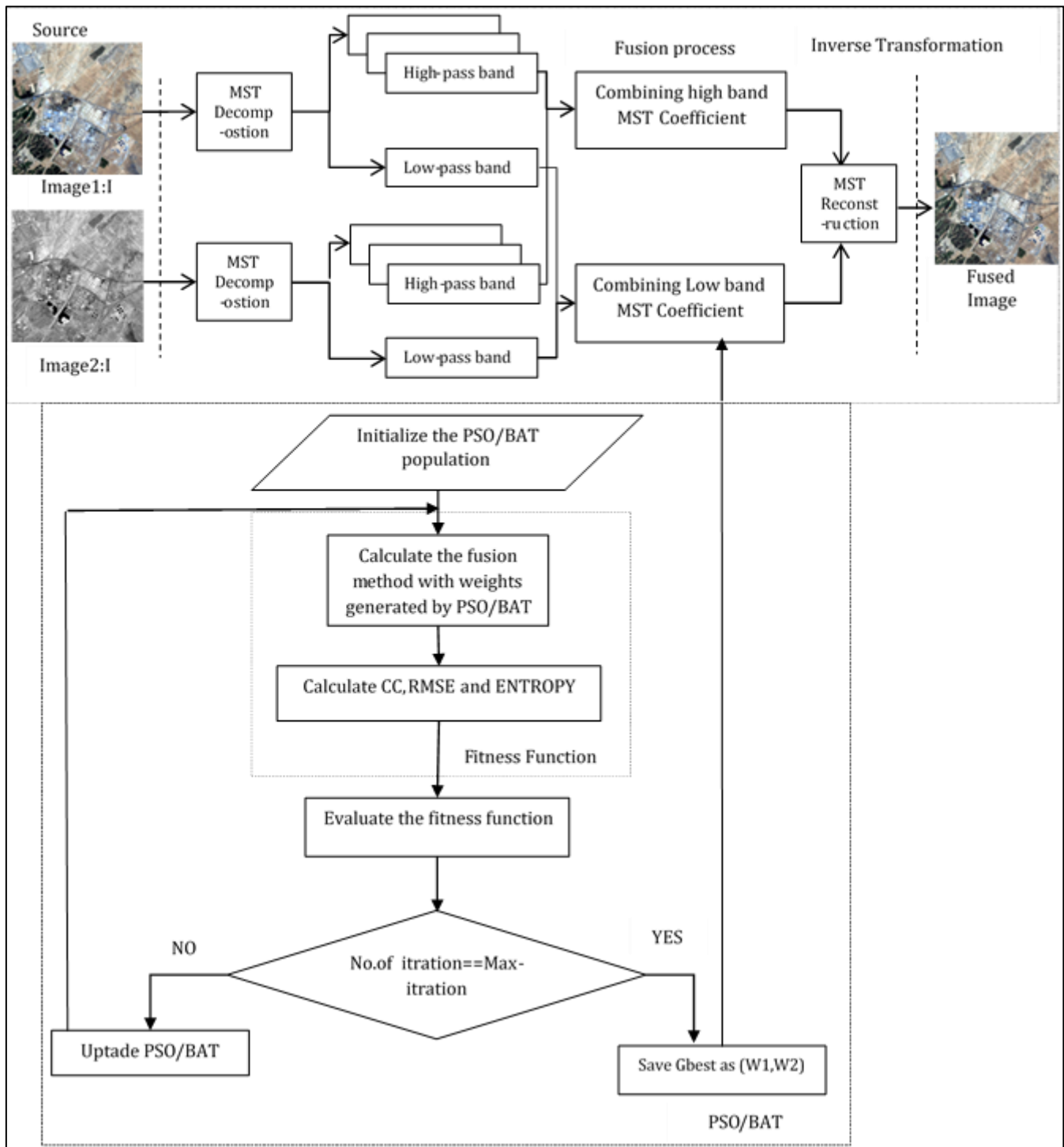
Figure 1. The image fusion process step with PSO and BAT algorithms
