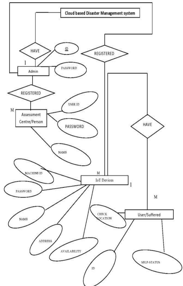
Figure 2. ER-Diagram
