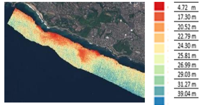
Figure 4. ln (blue) / ln (green) forecast bathymetry map
