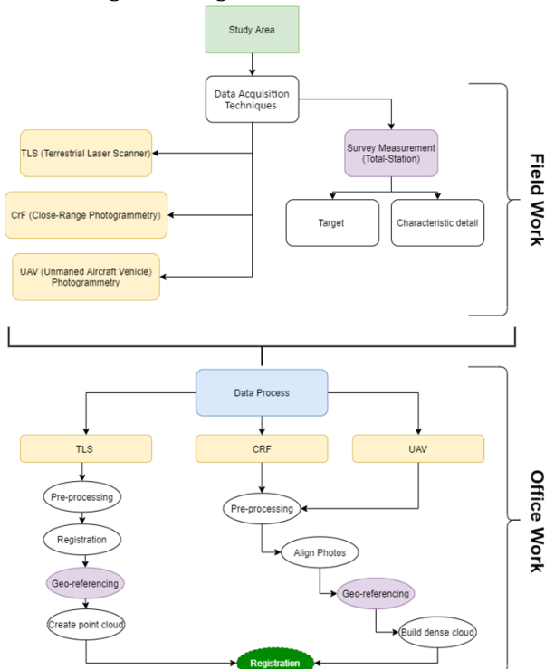
Figure 1. Workflow Chart
