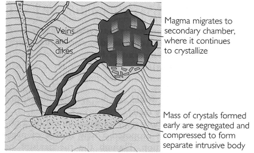
(b) Later deformation squeezes remaining liquid from crystal mush
