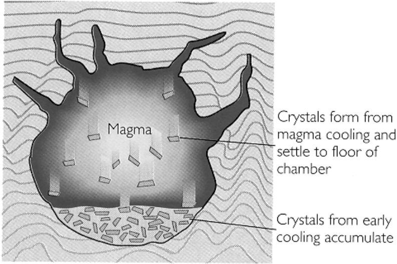
(a) Early crystallization
