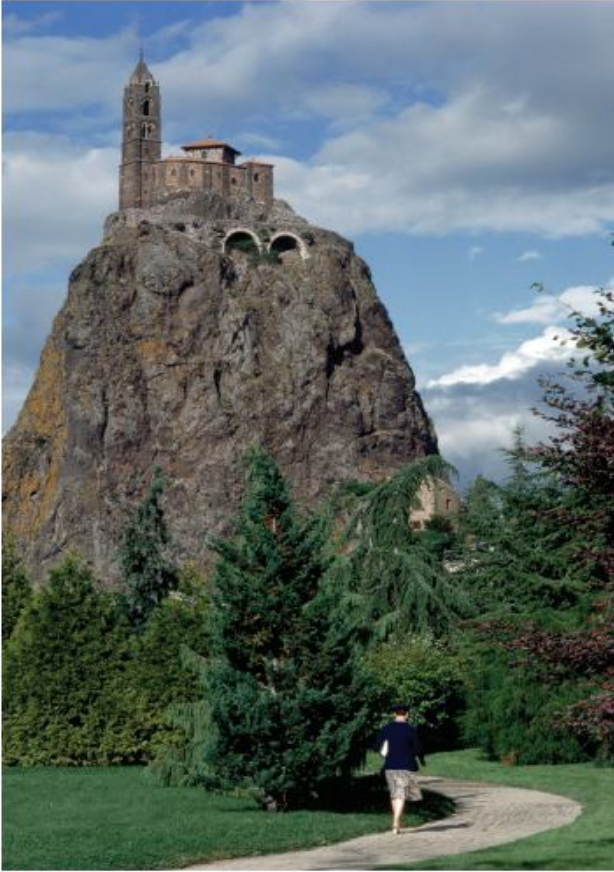
Volkan boynu
